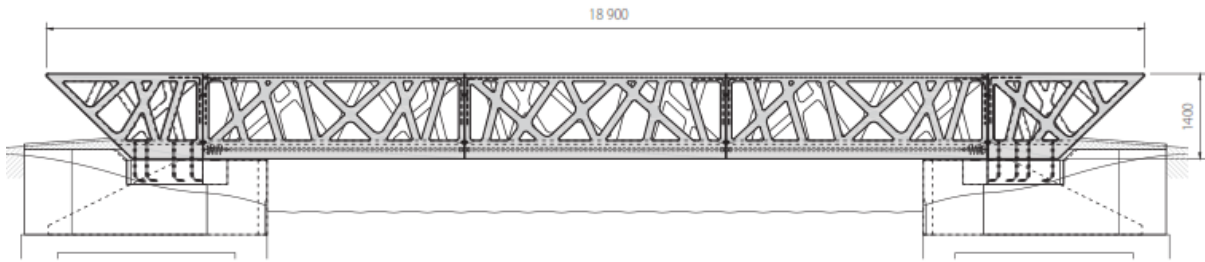
Figure 2: Side view of the bridge
