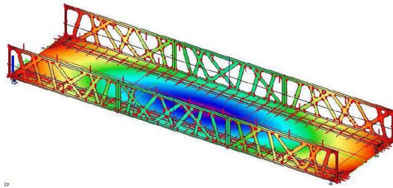
Figure 8: 3D model – vertical deflections [2]
