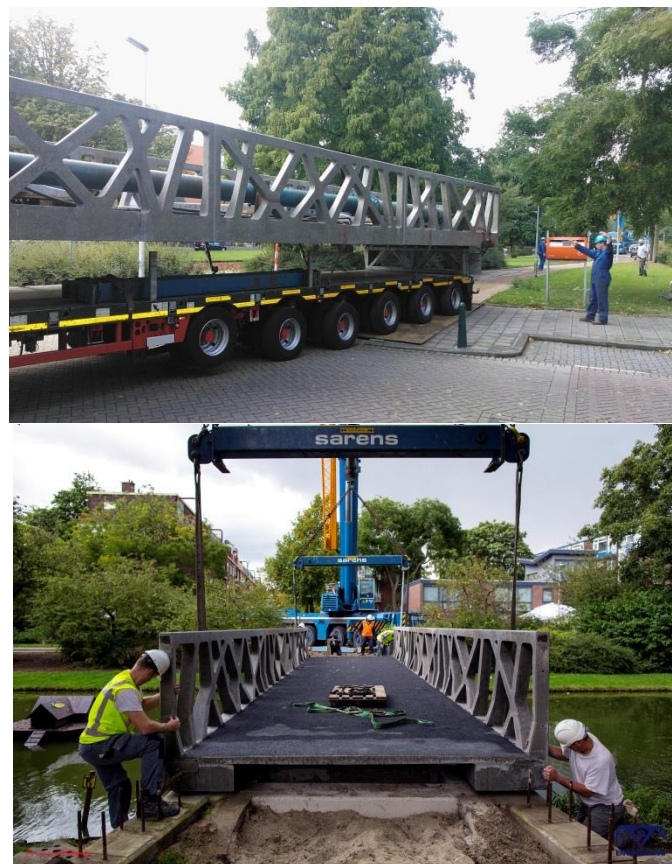
Figure 7: Transport of the bridge and installation at the definite location
